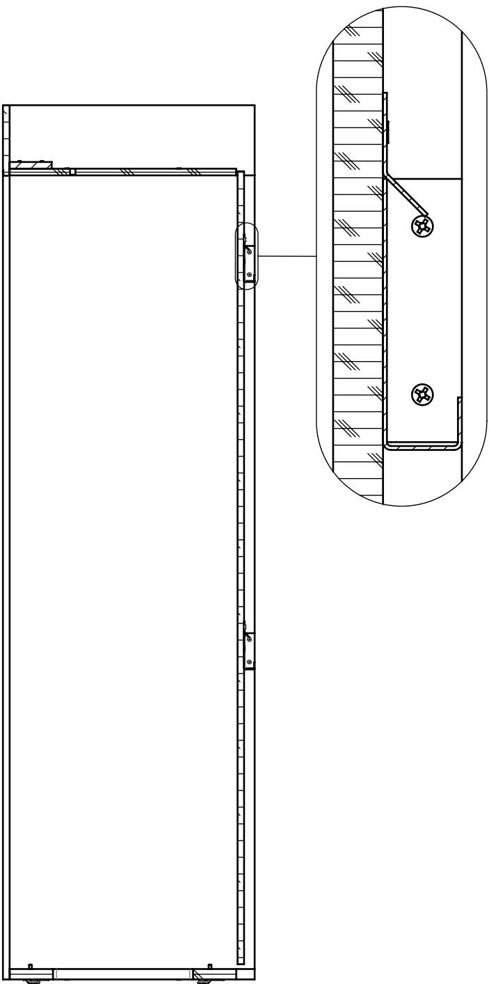
SECTION B-B
